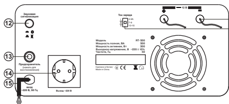
Fig. 3. Rear panel of RT-500
