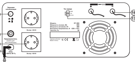
Fig. 4. Rear panel of RT-800*
